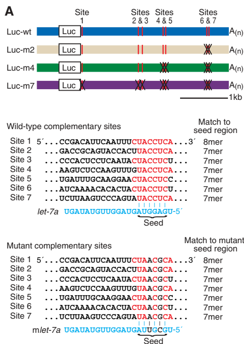
Fig. 2. Luciferase reporter assays showing the influence of miRNA-target pairing. (A) Design of Luciferase constructs. The 3' UTR of murine Hmga2 was appended to the Luciferase ORF (Luc). let-7 complementary sites are indicated (vertical red lines), as are mutant sites (black Xs). The Luc-m7, Luc-m4, and Luc-m2 were identical to Luc-wt, except they had seven, four, and two mutant sites, respectively. Each mutant site had two point substitutions that disrupted pairing to let-7 but created pairing to mutant let-7 ( mlet-7 , bottom, in blue). The seven sites were identified in a search for conserved 7- and 8-nucleotide motifs (7mer and 8mer) matching the seed region of let-7 (15). (B) Reporter repression in F9 cells supplemented with the indicated miRNA. Bars are colored to indicate the number of sites mutated in the reporter. Shown are median repression values, with error bars indicating 25th and 75th percentiles; n = 12, except experiments with no added miRNA (–), in which n = 36. Within each quartet, activity was normalized to that of the Luc-m7 reporter, except for the mlet-7 quartet, for which activity was normalized to that of the Luc-m7 reporter with noncognate miRNA (miR-124). (C) Reporter repression in NIH3T3 cells (top) or HeLa cells (bottom) supplemented with the indicated miRNA, performed and displayed as in (B). We also noticed two additional let-7 complementary sites in the murine Hmga2 mRNA, but located in the 5' UTR. When tested in luciferase reporter assays, these sites mediated little or no repression in the different cell lines, and the mutant sites did not respond to mlet-7 , indicating that any effects observed with the 5' UTR sites were not miRNA specific.
